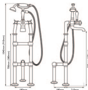
Freestanding Mixer Taps, With Standpipes, Ceramic Disc Valve
